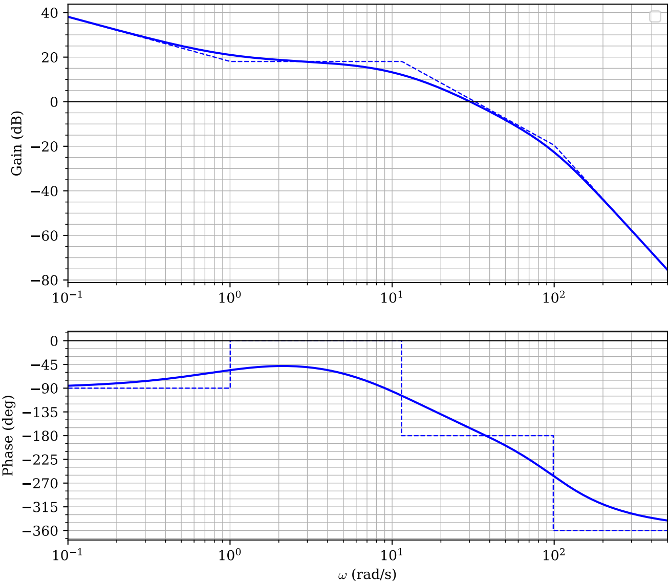
FIGURE 1 – Bode de la FTBO non corrigée — K_i = 1
